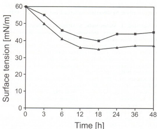
Figure 2. Kinetics of surfactant production of strain 2P of Bacillus licheniformis . Biosurfactant activity as determined by measuring changes in surface tension under aerobic (▲) and anaerobic (■) conditions as described by Yakimov et al. 1997 [21].
