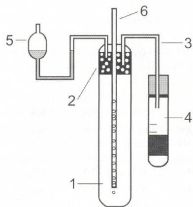
Figure 1. Laboratory column used for the evaluation of selected bacterial cultures based on oil recovery. (1) Column full with saturated sand oil; (2) Fiber buffer for filtration of mobilized fluids; (3) Oil and gas tube collector from the microbial recovery process; (4) Collector with a scale to measure recovered oil; (5) Special collector to indicate gas formation; (6) Sample injector.
